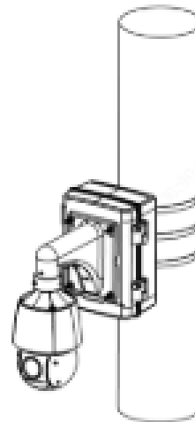
Pole Mount XLGUP08A + XLGJB12 + XLGWE45
